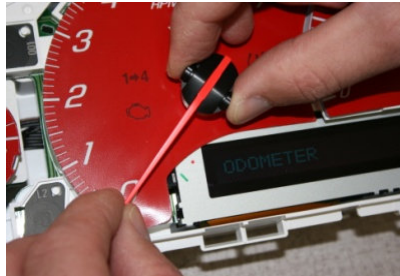
21. If a needle is set wrong, remove it. Unplug the cluster and start over.
