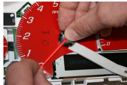
22. Place the cluster on a flat surface and press the needles down.
