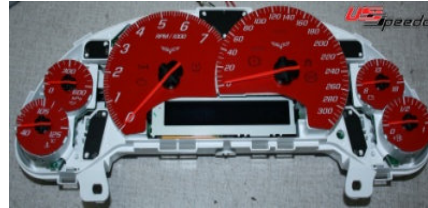
18. Now you should have all the needles in place. Unplug and put the cluster in your lap.
